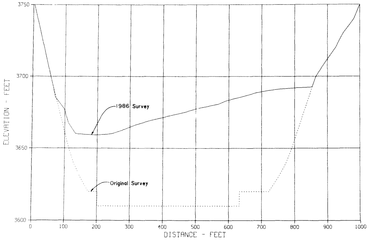
Figure 32. – Original and 1986 sedimentation range profiles, range 352, Colorado River.
