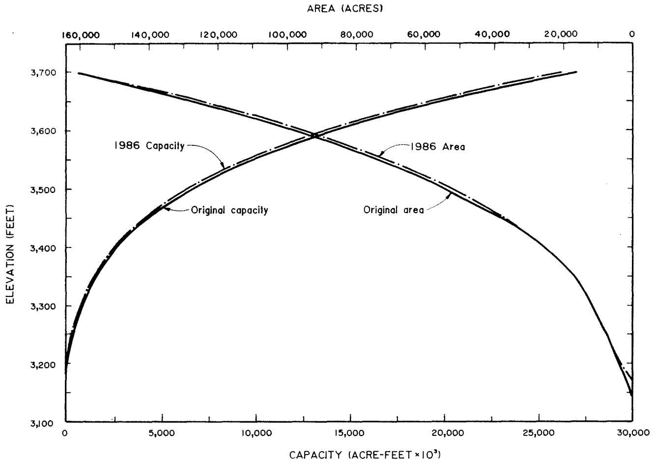
Figure 13. – Area and capacity curves.
