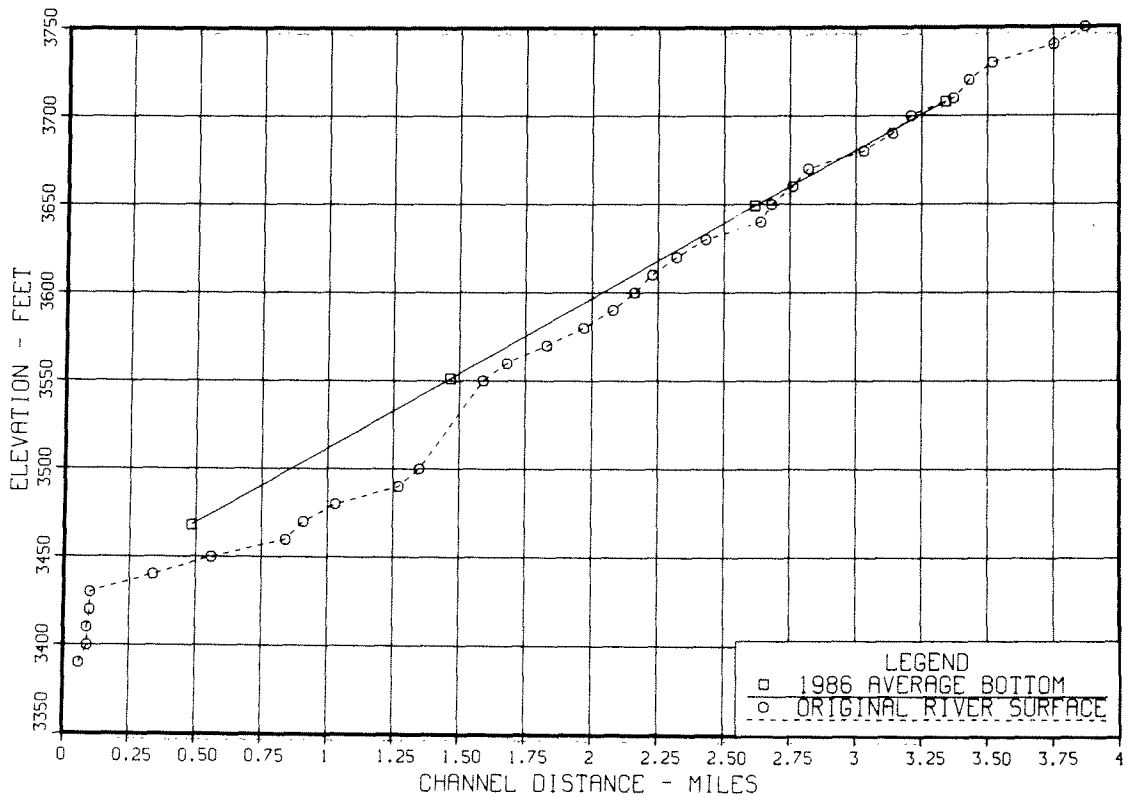
Figure 48. - Cedar Canyon profiles.
