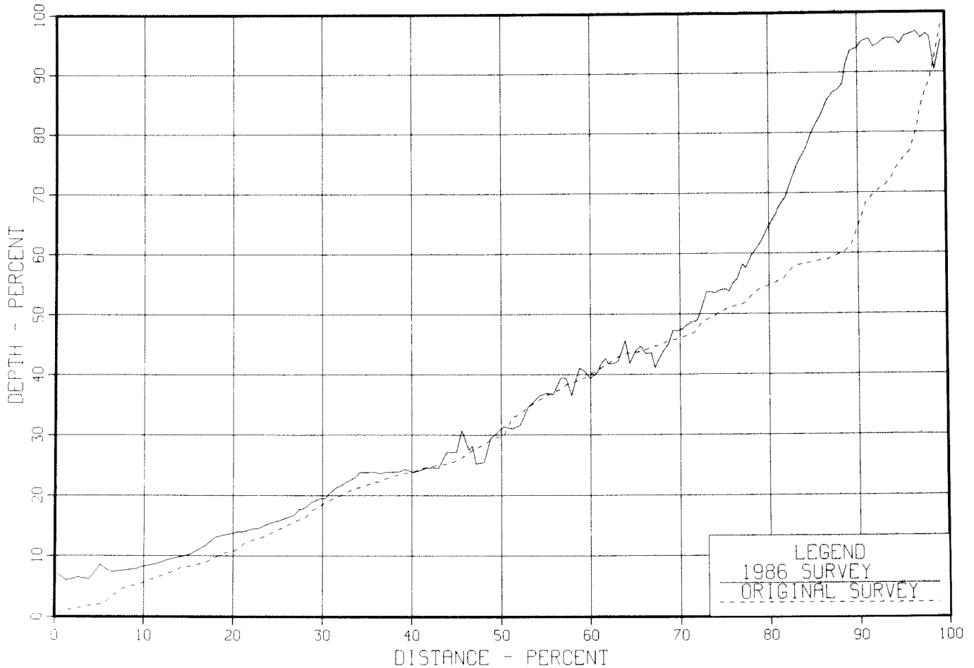
Figure 16. - Percent depth versus percent distance for Lake Powell above Glen Canyon Dam.
