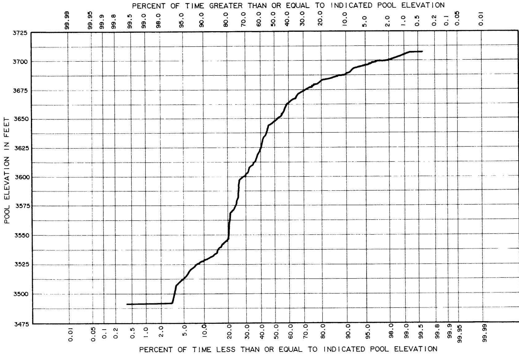
Figure 20. - Reservoir stage duration curve.
